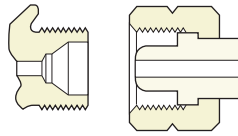
Connection 555 0.903" – 14NGO LH EXT.
