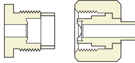
Connection 634 1.03" – 14NGO RH EXT.
