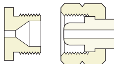
Connection 677 1.03" – 14NGO LH EXT.
