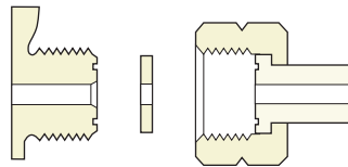
Connection 330 0.825" – 14 LH EXT., with Gasket
