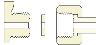
Connection 320 0.825" – 14 RH EXT., with Gasket
