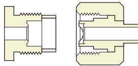
Connection 640 1.03" – 14NGO RH EXT.
