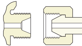
Connection 300 0.825" – 14 NGO RH EXT.
