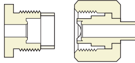
Connection 724 1.125" – 14NGO RH EXT.
