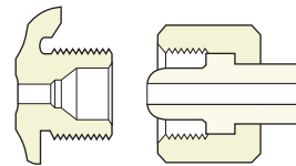
Connection 346 0.825" – 14 NGO RH EXT.
