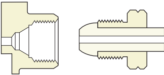
Connection 590 0.965" – 14NGO LH INT.
