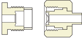
Connection 722 1.125" – 14NGO RH EXT.
