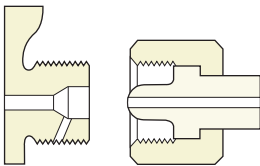
Connection 326 0.825" – 14 RH EXT.
