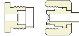
Connection 636 1.03" – 14NGO RH EXT.
