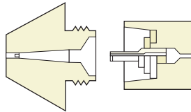
Connection 600 1" – 20 UNEF RH EXT., with Gasket
