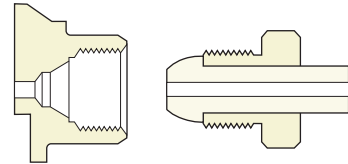
Connection 580 0.965" – 14 RH INT.
