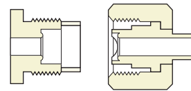
Connection 720 1.125" – 14NGO RH EXT.
